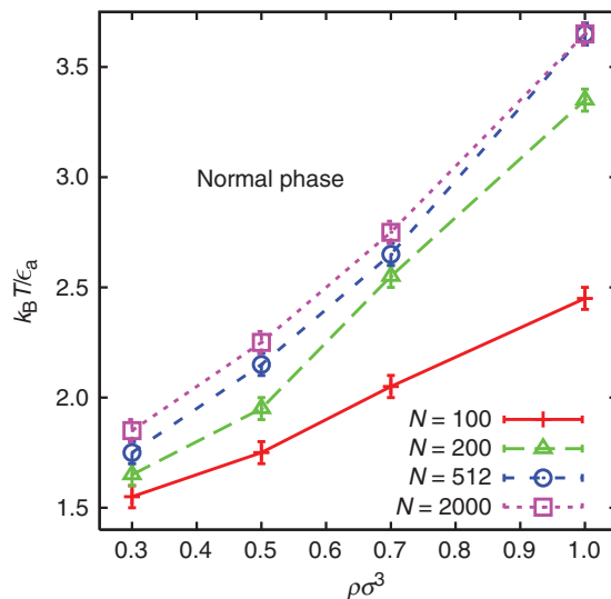
Figure 6. Size dependence of the instability line of Figure 5 for the system \epsilon_a/\epsilon_r=1/4 and \Delta/\sigma=0.5 .
