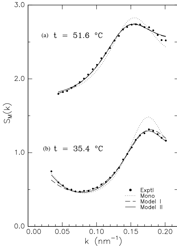
Fig. 2. Fit of experimental neutron scattering data for S_M(k) at \eta = 0.28 and two different temperatures (taken from Ref. [3]), by using monodisperse and polydisperse SHS-MSA models (the curves of part (a) are shifted upwards by 2.5 units).
