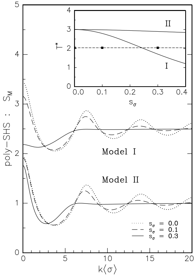
Fig. 1. Structure factor S_M(k) of the SHS-MSA Models I and II at T^* = 2.04 and \eta = 0.2 , for several degrees of polydispersity s_\sigma (the curves of Model I are shifted upwards by 1.5 units to avoid overlapping). In the inset, the solid curves represent T_{B,F}^*(s_\sigma) of the two Models, the dashed line corresponds to the isotherm T^* = 2.04 and the black squares on it are the considered states.
